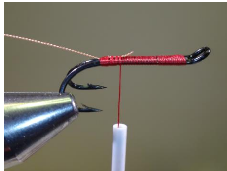
2. Tie in the twisted copper wire
