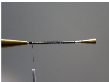
1 Tie in the thread and wind it in close turns to the end of the tube
